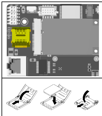
Fig. 5-3 inserting the SIM card
